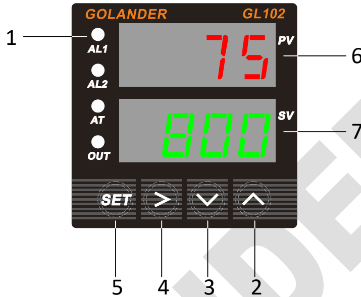
Figure 2 Front Panel
