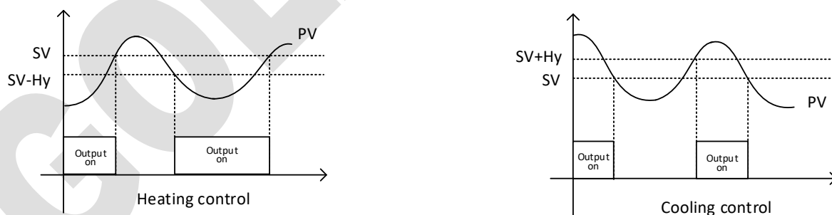
Figure 4. on/off control
