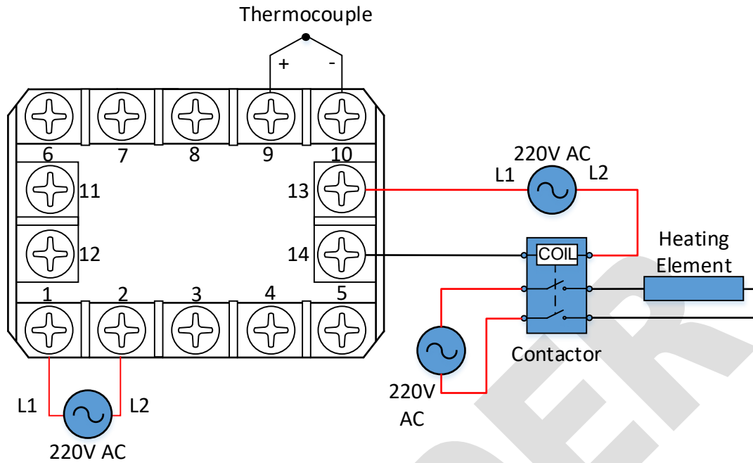
Figure 7. Use Contactor for Heater
