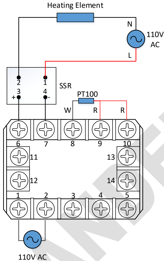
Figure 6. Heater Wiring
