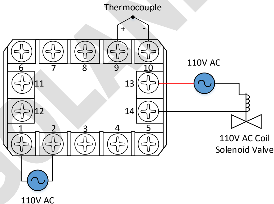
Figure 5. 110V AC Solenoid Valve Wiring
